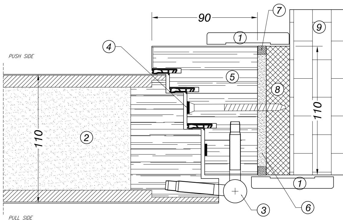
FRAME-LEAF DETAIL - INSTALLATION ON WALL
