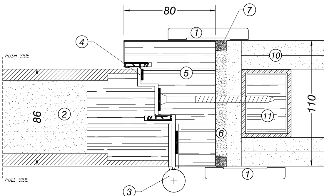
FRAME-LEAF DETAIL - INSTALLATION ON PLASTERBOARD
