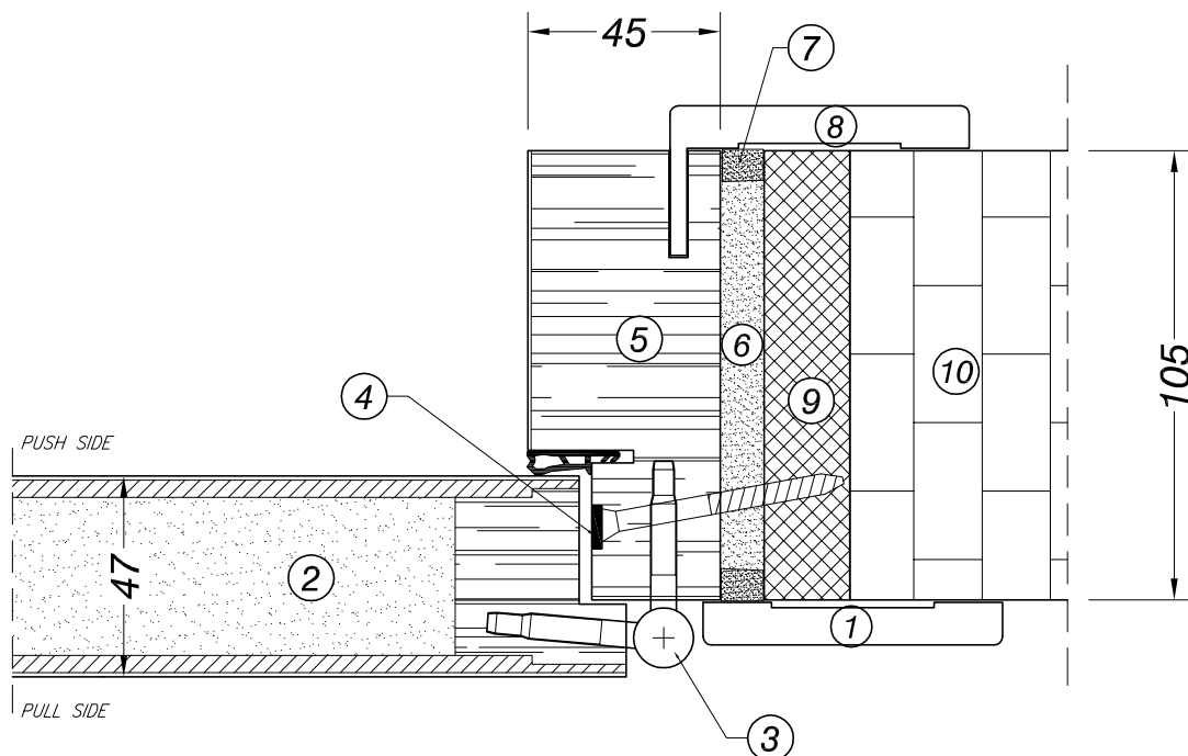
FRAME-LEAF DETAIL - INSTALLATION ON WALL
