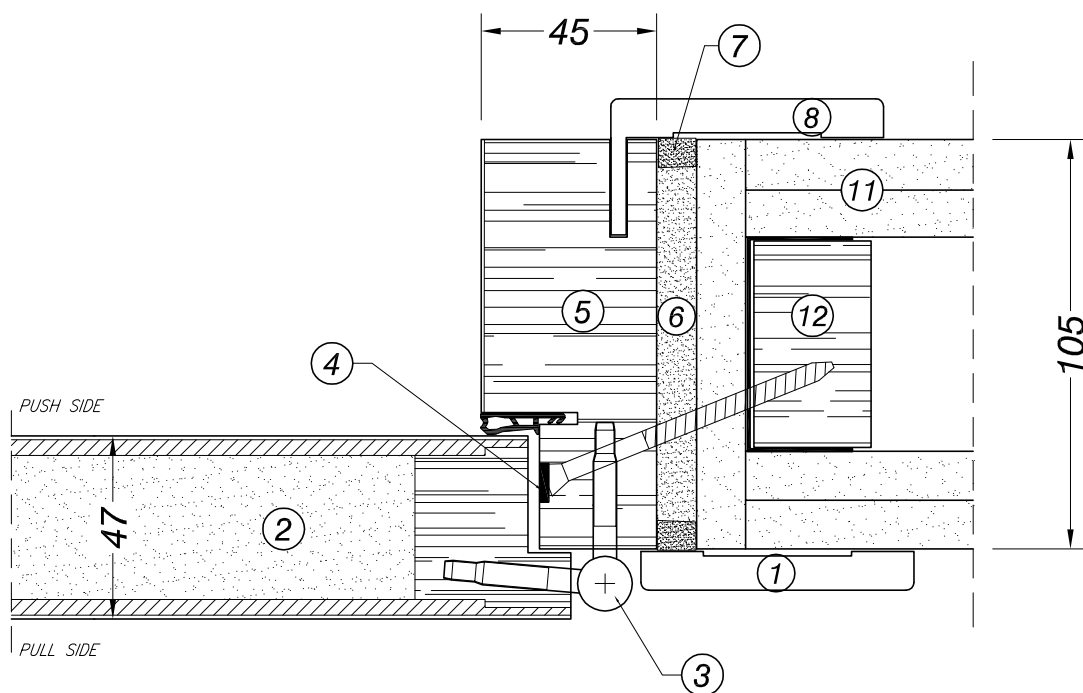
FRAME-LEAF DETAIL - INSTALLATION ON PLASTERBOARD
