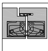
CONCEALED HINGE
