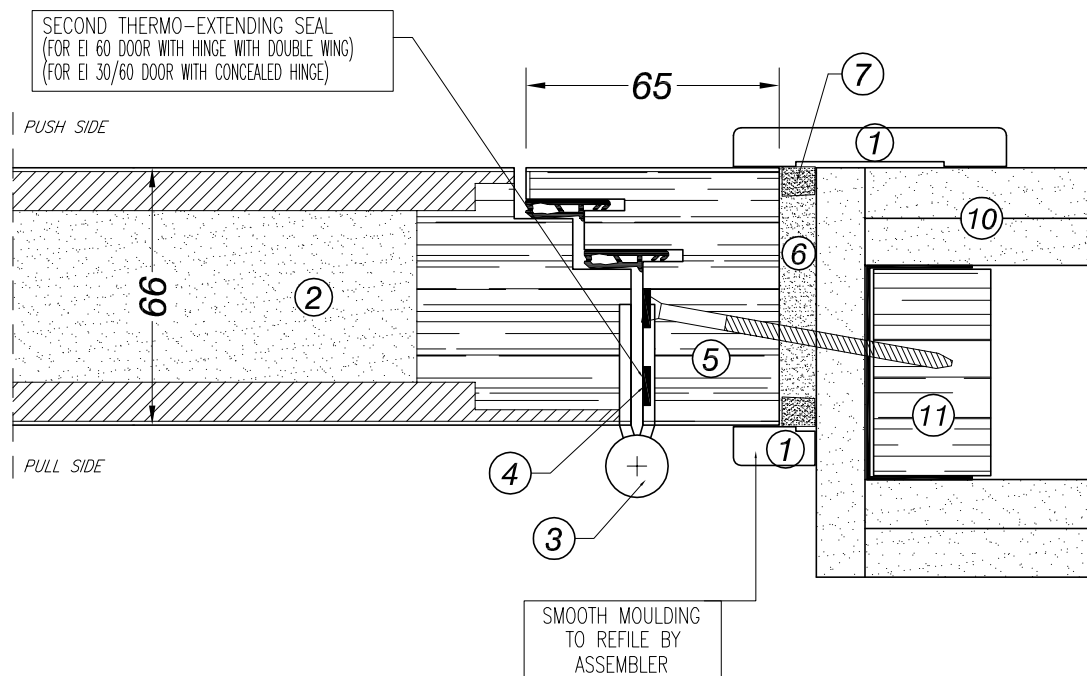
FRAME-LEAF DETAIL - INSTALLATION ON PLASTERBOARD
