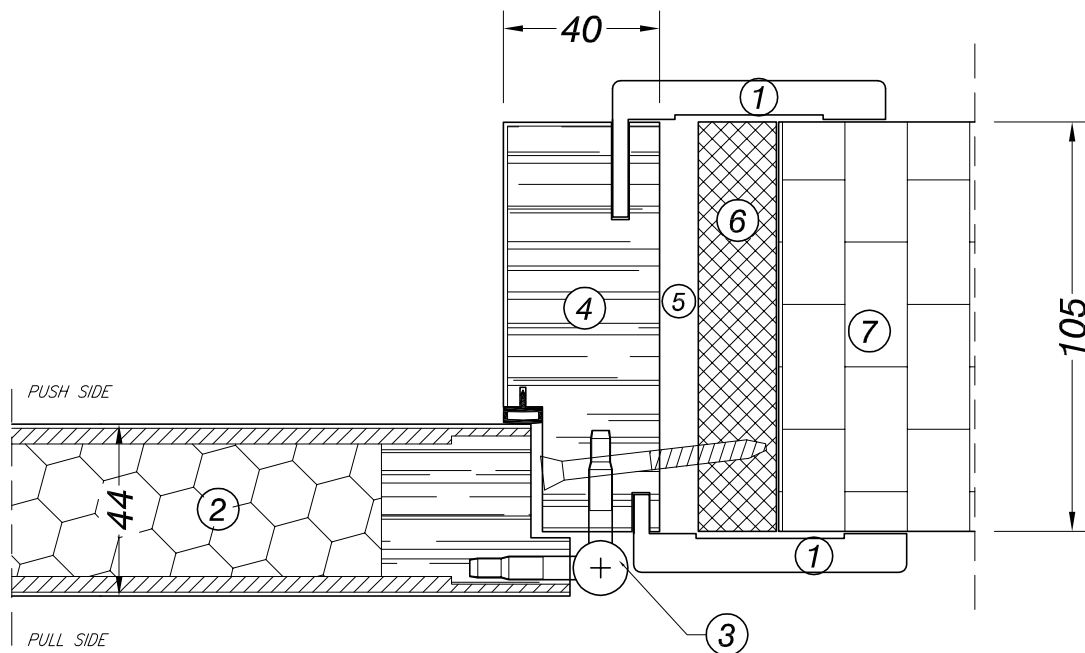
FRAME-LEAF DETAIL - INSTALLATION ON WALL
