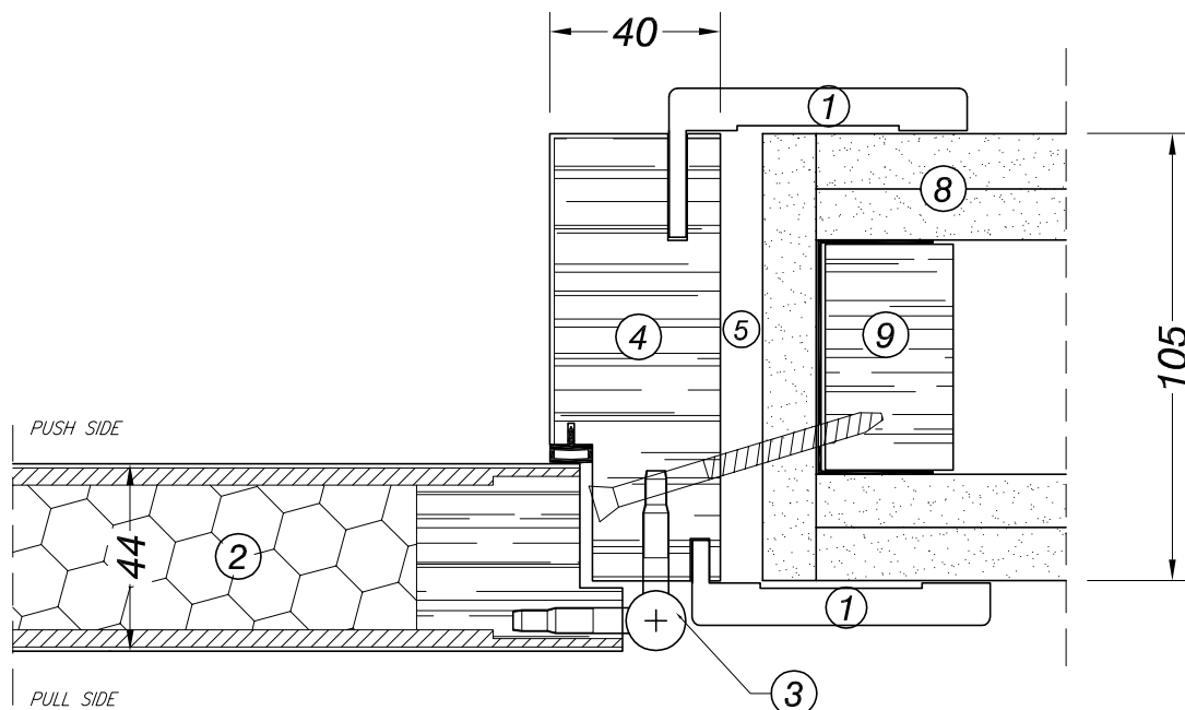
FRAME-LEAF DETAIL - INSTALLATION ON PLASTERBOARD
