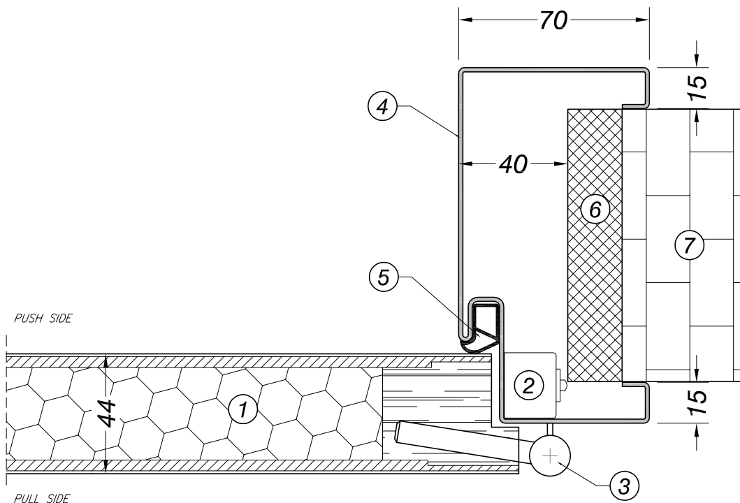
FRAME-LEAF DETAIL - INSTALLATION ON WALL
