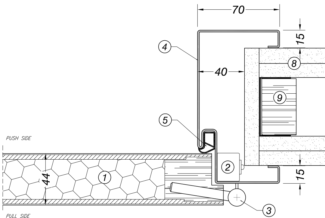
FRAME-LEAF DETAIL - INSTALLATION ON PLASTERBOARD
