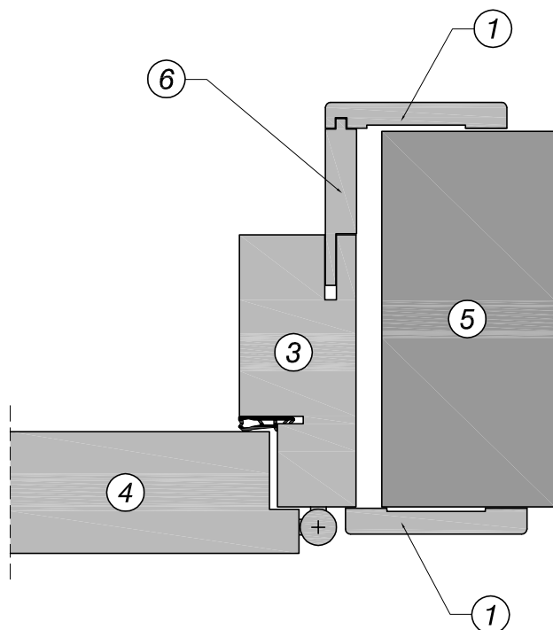
GENERAL PLACEMENT RABBET LEAF DOOR WITH STANDARD WALL COVER
