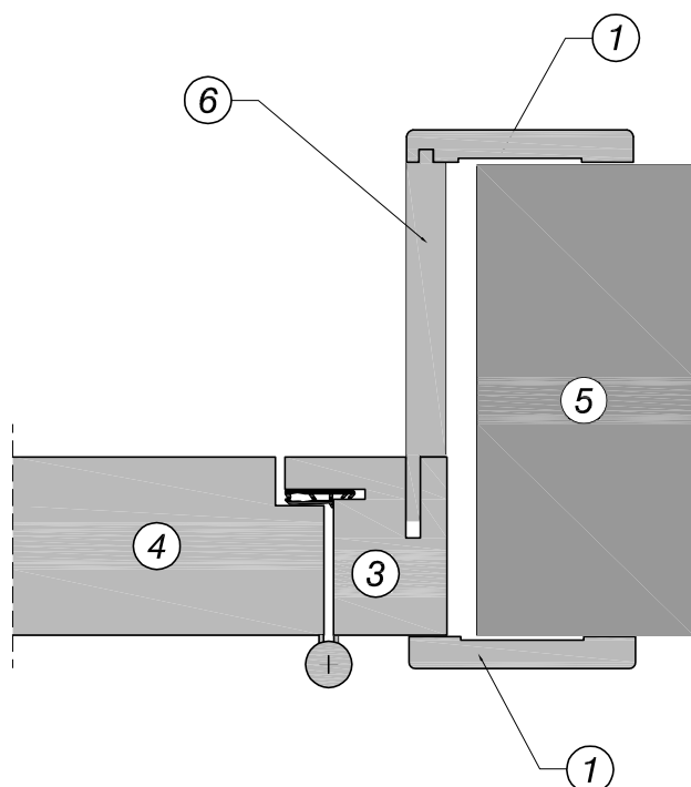
GENERAL PLACEMENT FLUSH LEAF DOOR WITH STANDARD WALL COVER
