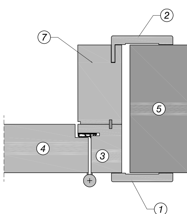
GENERAL PLACEMENT FLUSH LEAF DOOR OPTIONAL VERSION WITH FRAME EXTENSION
