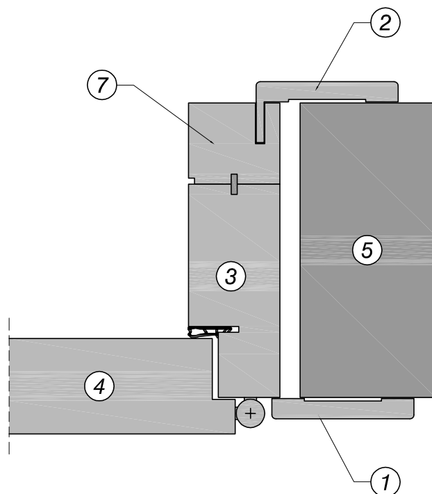
GENERAL PLACEMENT RABBET LEAF DOOR OPTIONAL VERSION WITH FRAME EXTENSION
