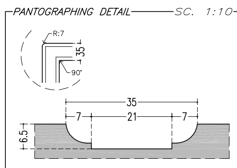
PNT D Thickness : 6.5mm_35(7+21+7)
