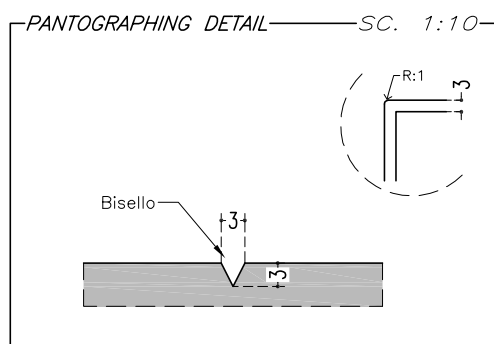
PNT A Thickness : 3 x 3 mm
