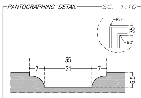
PNT C Thickness : 6.5mm_35(7+21+7)
