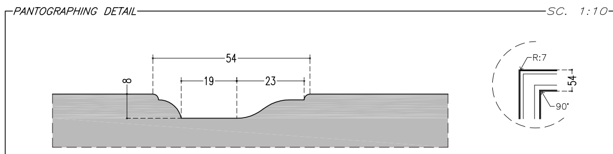
PNT E Thickness : 8mm_54(2+8+19+23+2)
