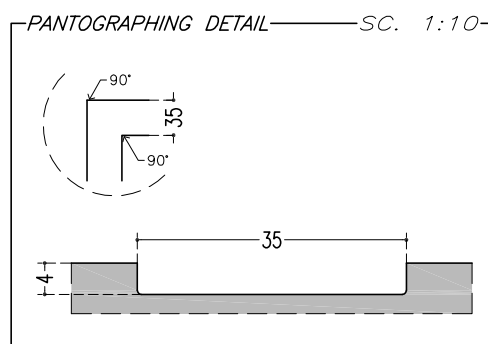
PNT B Thickness : 4 x 35 mm
